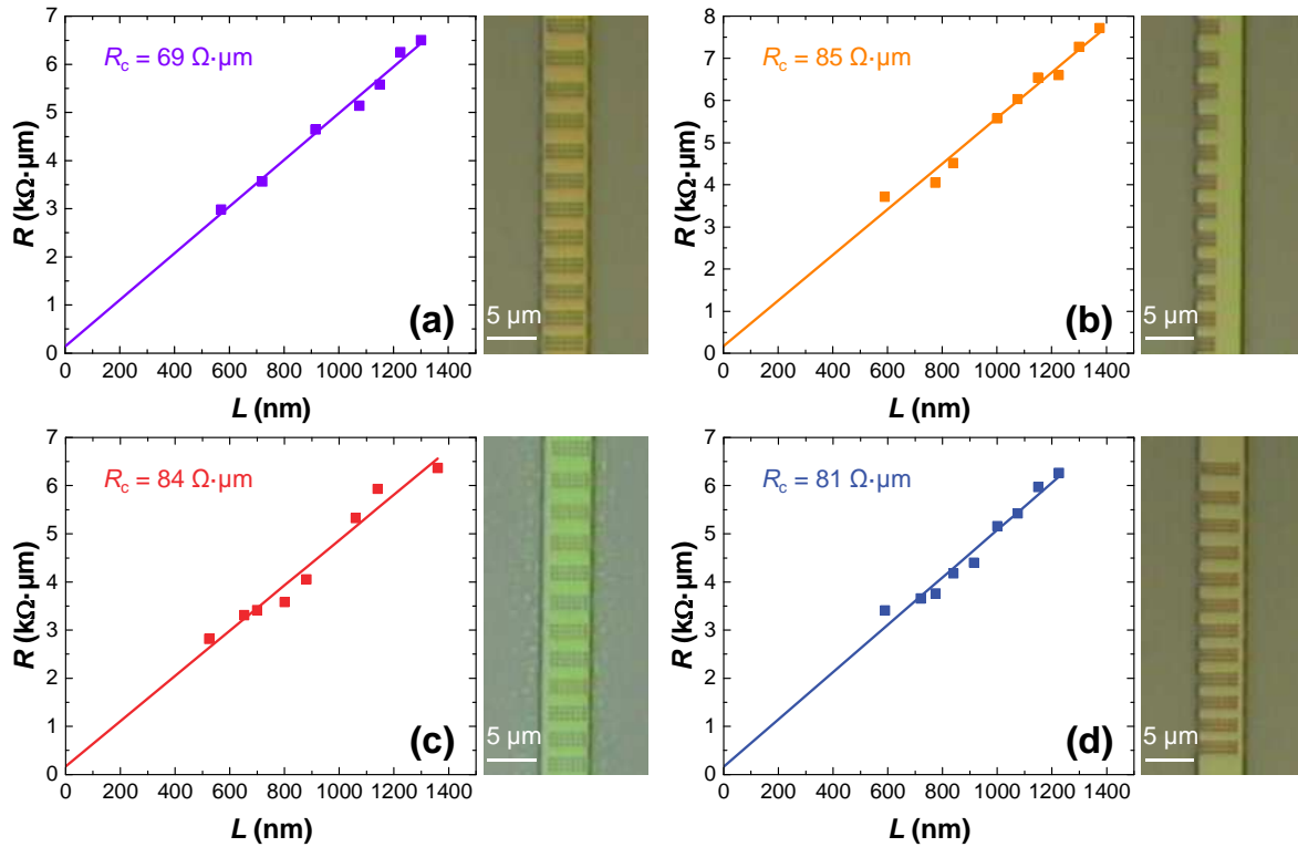
Figure S1. Contact resistance in holey graphene TLM devices with a different degree of hole misalignment. For each device, the linear fit of the resistances between the contacts at the Dirac point and an optical image of the graphene channel after etching are shown. (a) The holes are not etched only across small areas close to the edges of the channel. (b) The holes are etched only across the left part of the channel. (c) The holes are not etched across the left edge of the channel. (d) The holes are not etched across the right edge of the channel.
