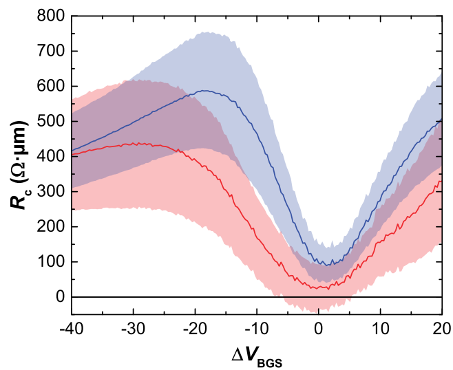
Figure S2. The contact resistance obtained from two different TLM structures with holey Au (100 nm) contacts as a function of the back-gate voltage overdrive. The bias was V_{DS} = 10 mV. The shaded areas show the standard error.
