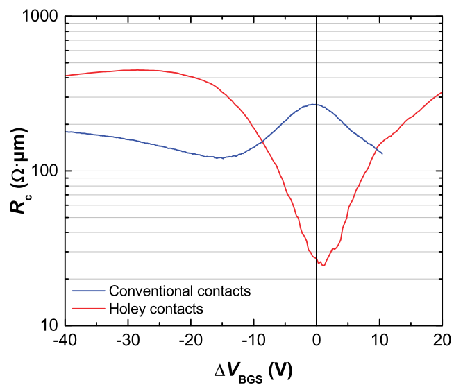
Figure S3. The contact resistance of a TLM structure without holes (blue) and with holes (red) as a function of the back-gate voltage overdrive. In both cases Au (100 nm) was used for the contacts and the bias was V_{DS} = 10 mV.
